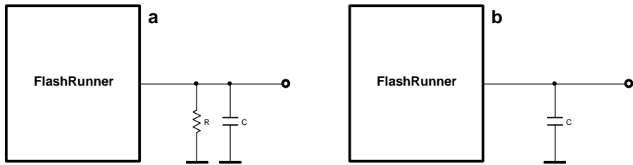
Figure 4.1: Load Conditions
